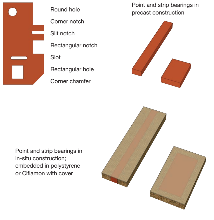
Fig. 4: Calenberg Compact Core Bearings, standard cut-outs and delivery forms
